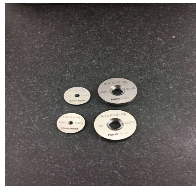
Thread Ring Gauge
