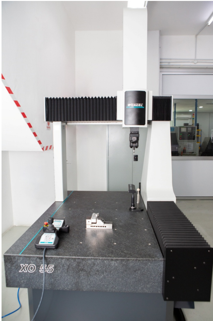
Wenzel Coordinate Measuring Machine (CMM) Model XO55-700. Measuring Range X=500 x Y=700 x Z=500mm
